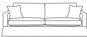
Three Seater Sofa CM W216 D100 H85
